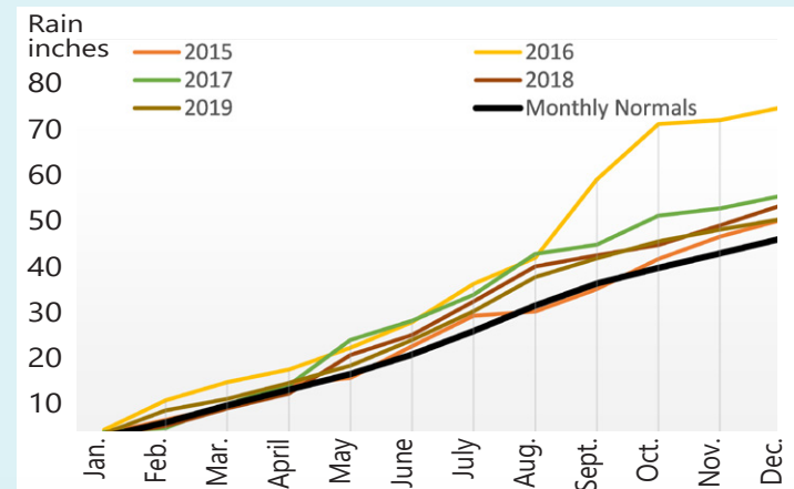
Cumulative monthly rainfall from Norfolk International Airport from 2015 to 2019. The black line is the long-term monthly normal average between 1981 and 2010. (Source: NOAA, National Climate Data Center)
