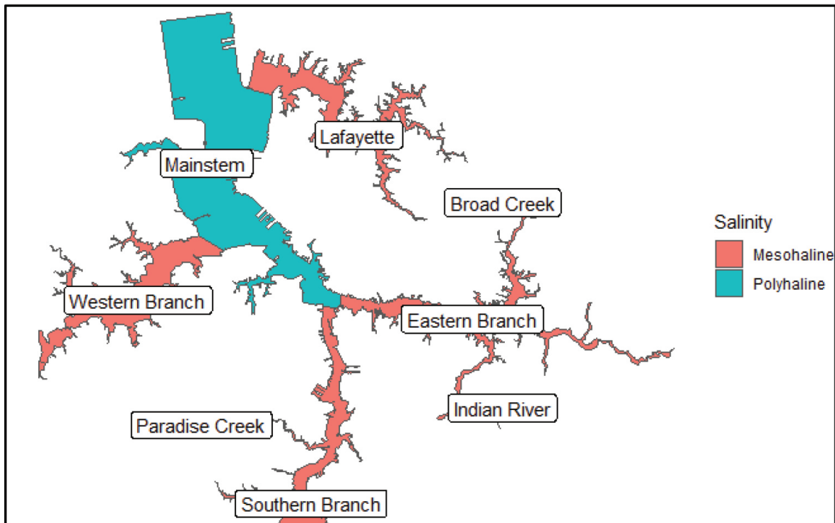
Figure 1: The Mainstem of the Elizabeth River is classified by the Polyhaline salinity regime. All other branches fall into the Mesohaline regime.
